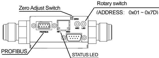
STATUS LED(NET,MOD)
