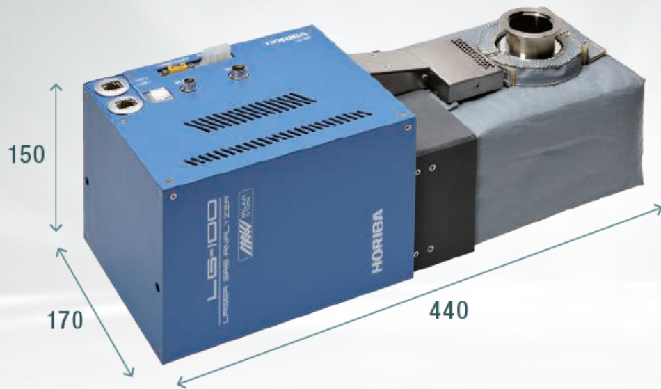
Sensor unit
