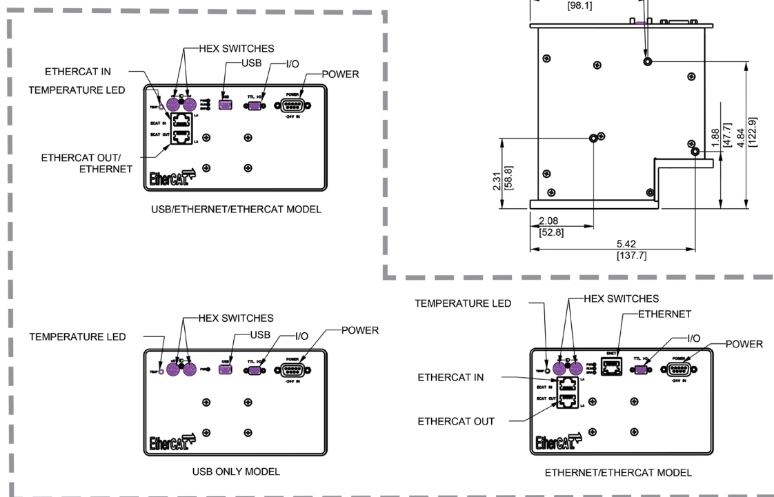
VS70-MC back panels for different models
