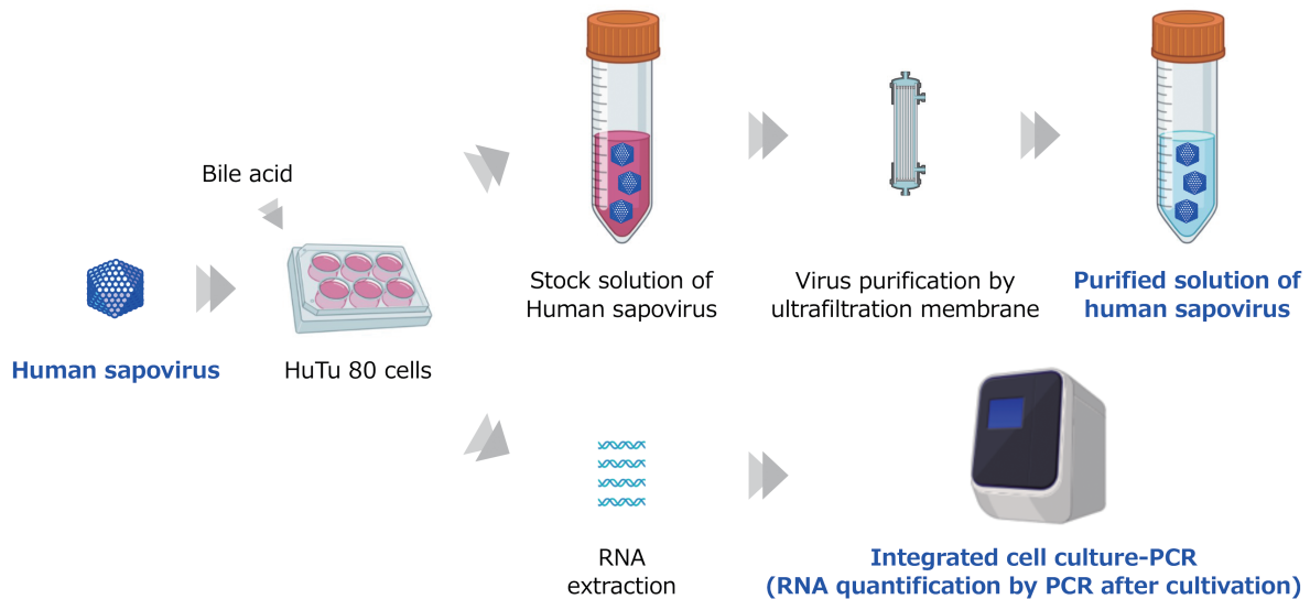
Figure 4 Schematic diagrams of preparation of purified human sapovirus solution and human sapovirus quantification by an integrated cell culture-PCR.
